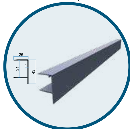
16mm F Profil 16mm F Profile Product Code: 2538 Weight kg/m: 0,210 (28,5 x 26 x 1mm)
