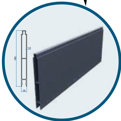
15x160 Lamela 15x160 Paneling Product Code: 2546 Weight kg/m: 1,591 (160 x 16 x 1,6mm)
