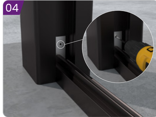
04 Fix L-clips to the post with self-drilling screws.
