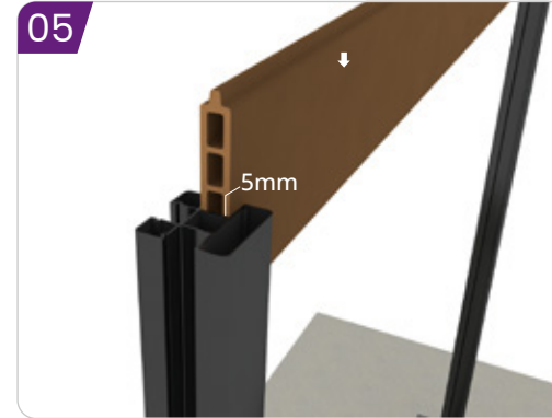
05 Slide the fence boards into the post slots in the correct direction, ensuring they are straight. Ensure a 5mm gap between the fence boards and posts.
