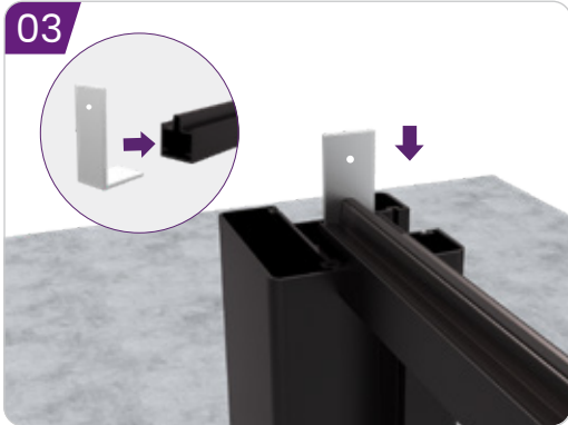
03 Attach L-clips to each end of the aluminum fence bottom rail and push them down to the bottom.
