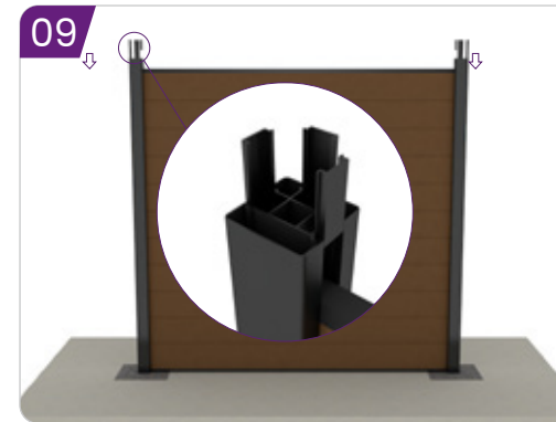
09 Slide in sealing edges.
